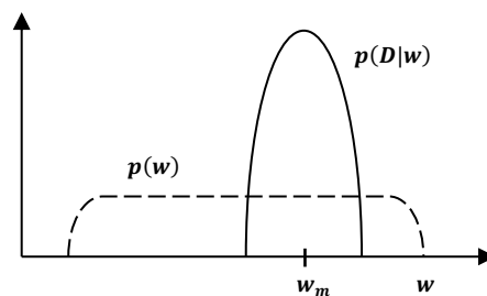
Fig. 2. Change pre weights to posterior/post weights [12]
