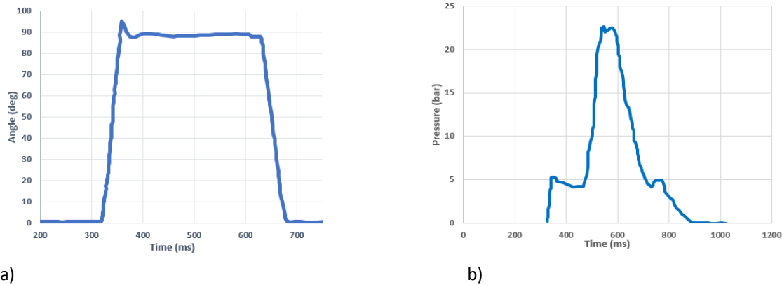
Fig. 13. a) The output response for shoulder abduction rotation b) The consumed pressure during shoulder joint movement
