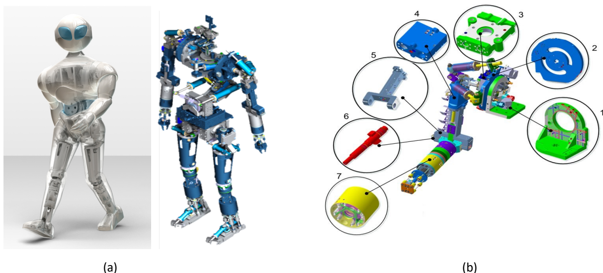
Fig. 1. a) HYDROiD robot CAD 3D model b) Overview on the arm hydraulic integrated parts masses: 1- Shoulder upper part, 2- Shoulder middle part, 3- Shoulder lower part, 4- Elbow upper part, 5- Elbow lower part, 6- Elbow axis of rotation, 7- Wrist part
