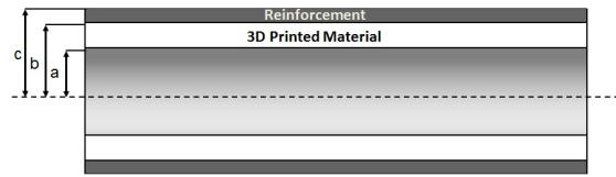
Fig. 4. Geometrical representation of the multilayer tube: (a) the internal diameter of the internal layer, (b) the internal diameter of the outer layer and (c) the outer diameter of the outer layer
