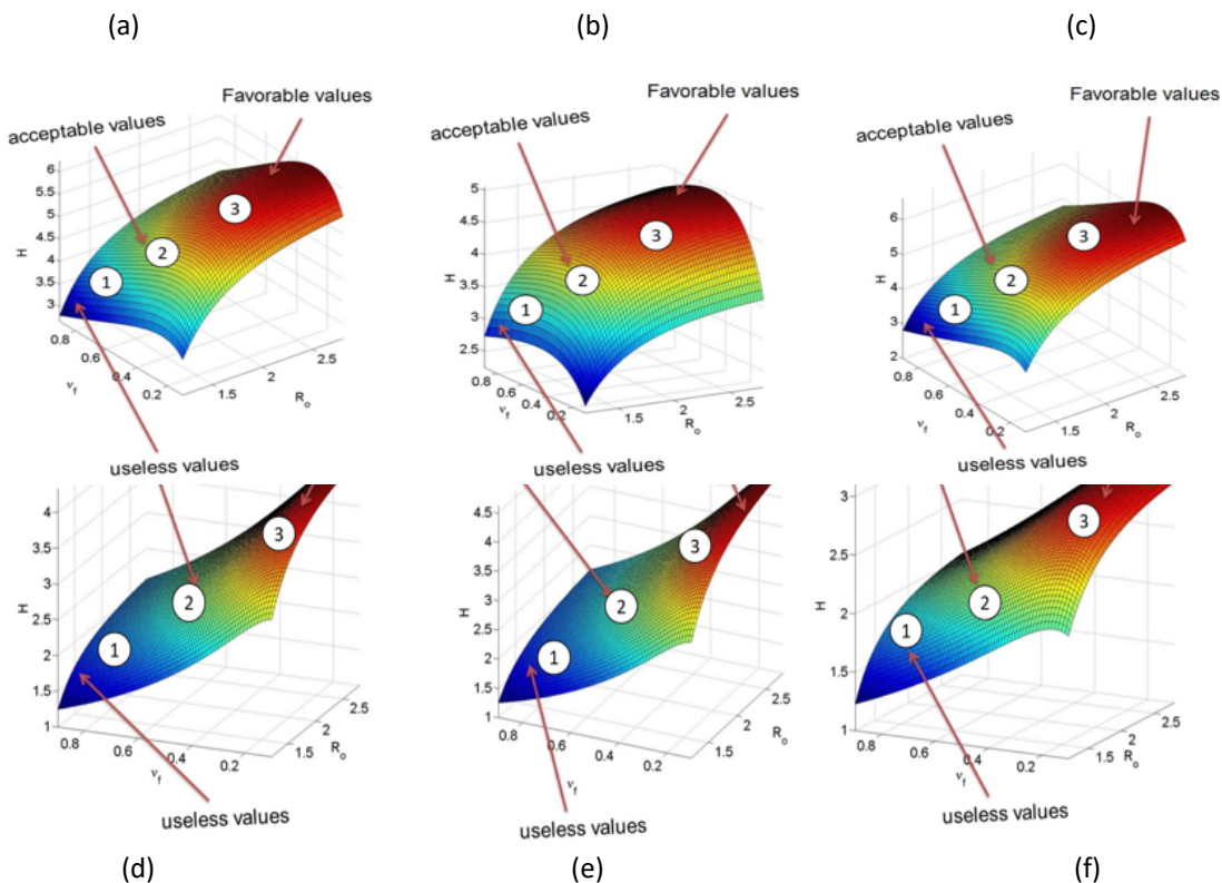
Fig. 6. Simulation results of function H for different materials like: (a)CF/Epoxy, (b)CF/Polyester, (c)CF/Polyurethane, (d) GF/Epoxy, (e) GF/Polyester and (f) GF/Polyurethane. Region 1 for useless values, region 2 for acceptable values and region 3 for favorable values
