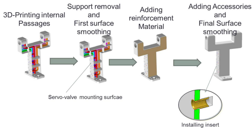
Fig. 3. Illustration of the procedure steps starting from internal passages printing ending with adding the accessories
