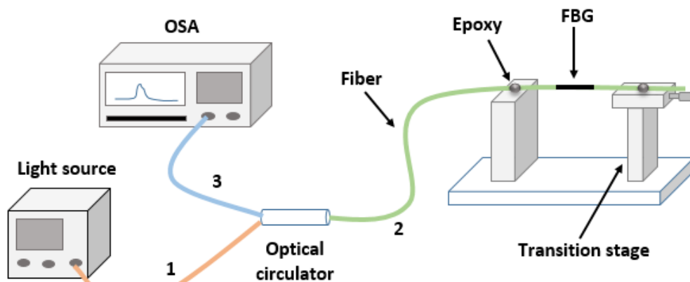
Fig. 1. Schematic experimental setup of strain sensor
