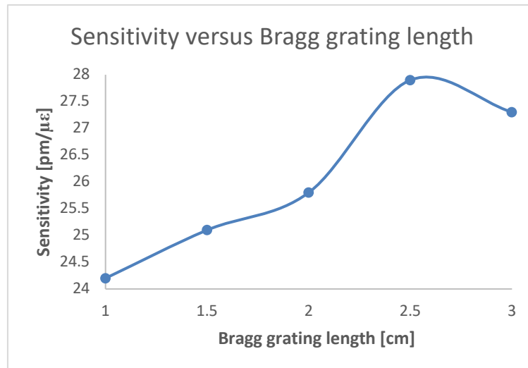
Fig. 6. Sensitivity versus Bragg grating length
