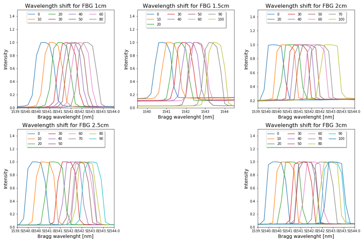
Fig. 4. Wavelength shift as a response to the increase of the strain on the FBGs
