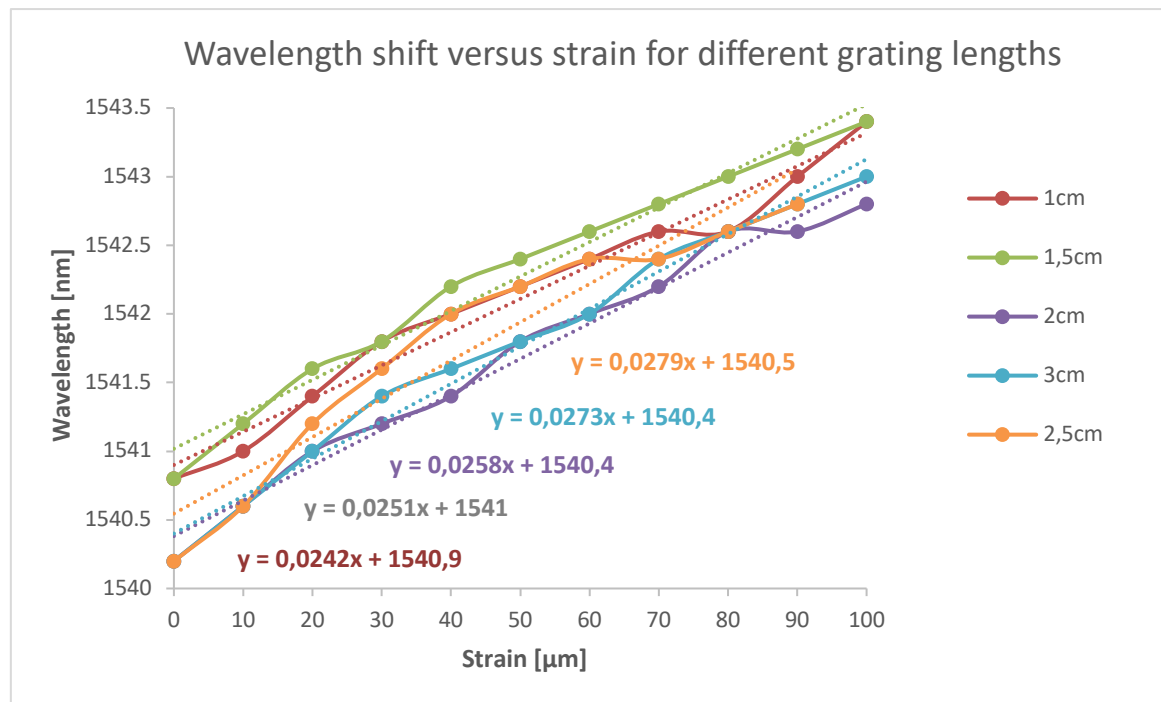
Fig. 5. Wavelength shift versus strain for different grating lengths
