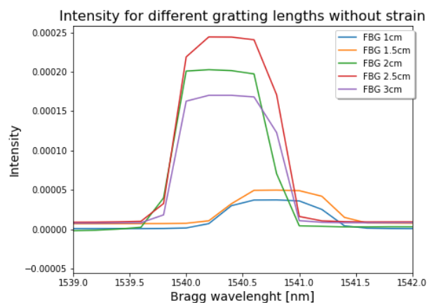
Fig. 3. Intensity for different grating length without strain
